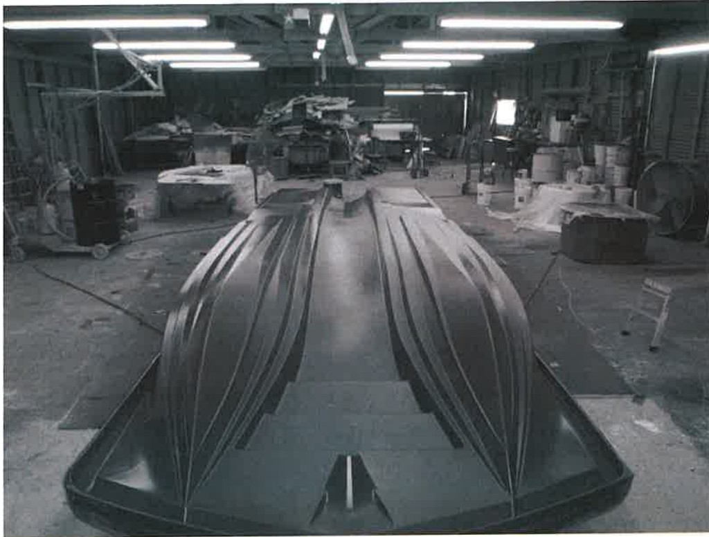
Transom View
